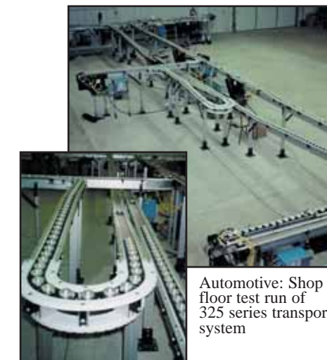
Automotive: 180-degree corner adapted for product accumulation
