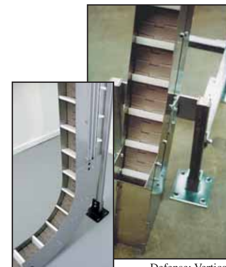
Defense: 90-degree vertical bend with a cleated 450 series segmented belt
